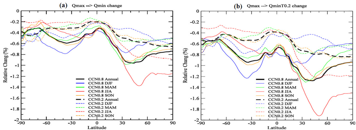
Figure 3. Annually and seasonally averaged zonal mean relative changes of CCN0.8 and CCN0.2 in the lower troposphere (0–3 km above the surface): (a) due to ionization rate change ( Q_{max} \rightarrow Q_{min} ) only; (b) due to both Q and T changes ( Q_{max} \rightarrow Q_{minT0.2} ). DJF (December, January, February), MAM (March, April, May), JJA (June, July, August), and SON (September, October, November) refer to winter, spring, summer, and fall seasons, respectively.
