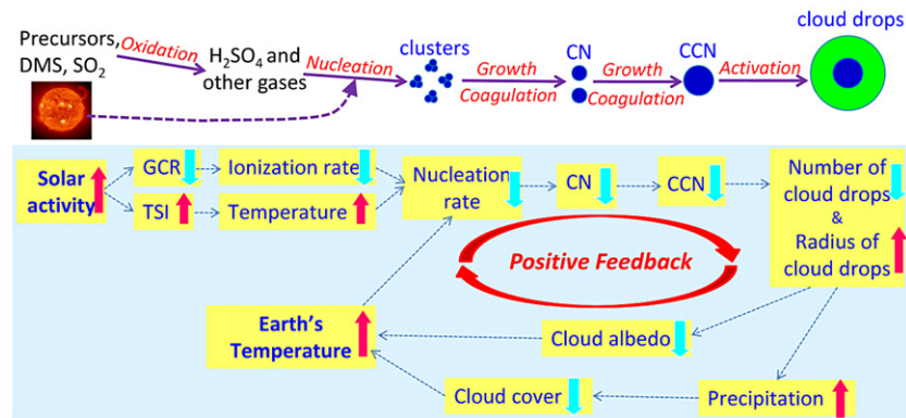
Figure 1. A schematic illustration of a mechanism amplifying the effect of solar variability through the influence of GCR ionization and temperature on particle formation and a positive nucleation feedback (enhanced solar activity → more TSI and less GCR → reduced nucleation and aerosol abundance → less aerosol cooling → increased temperature).
