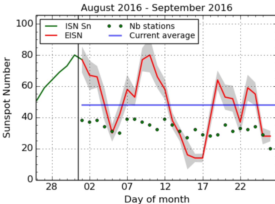
iILSO graphics ( http://sidc.be/silso ) Royal Observatory of Belgium, 2016 September 26
