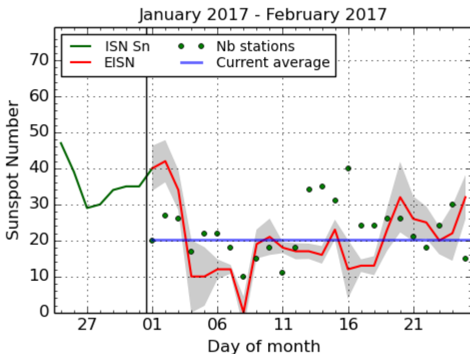
SILSO graphics ( http://sidc.be/silso ) Royal Observatory of Belgium, 2017 February 25
