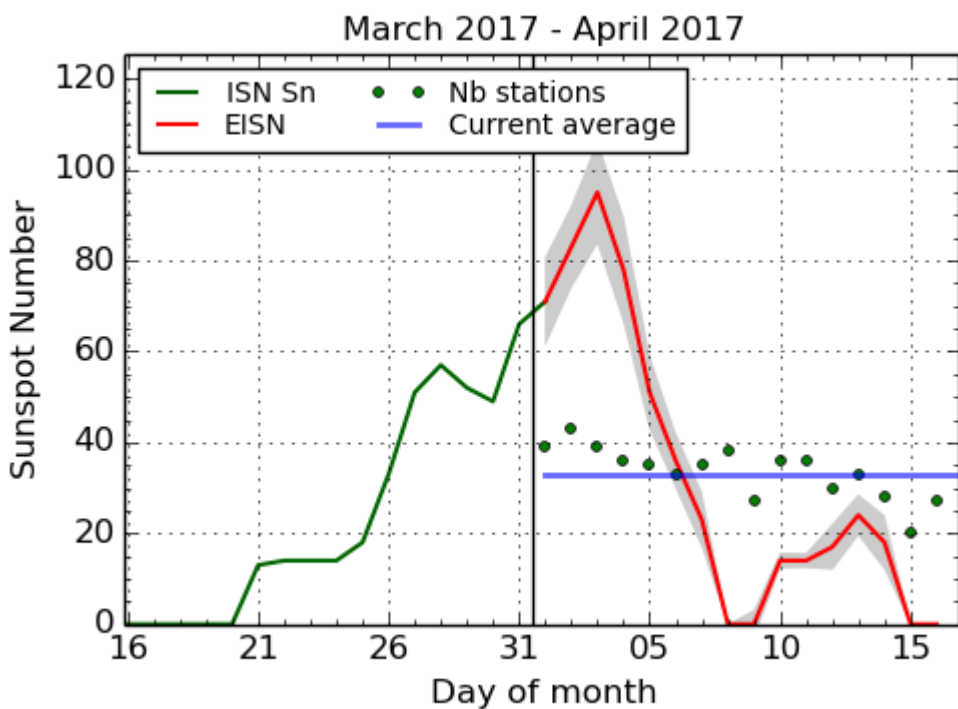
SILSO graphics ( http://sidc.be/silso ) Royal Observatory of Belgium, 2017 April 16
