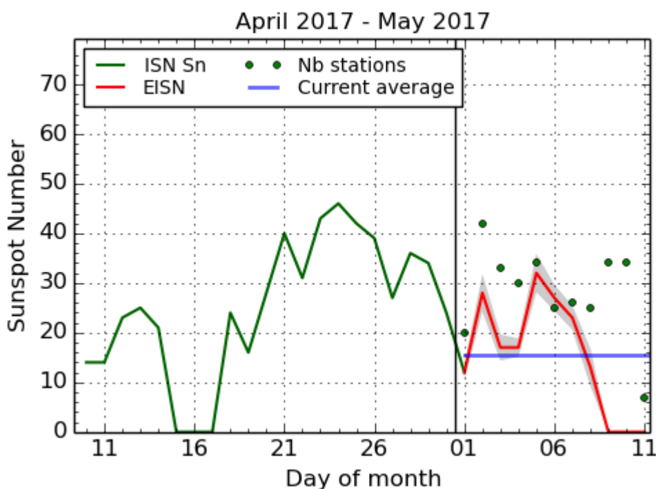
SILSO graphics ( http://sidc.be/silso ) Royal Observatory of Belgium, 2017 May 11
